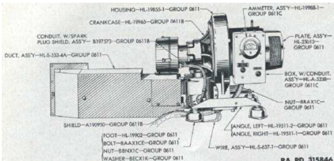
FIGURE 06-56—AUXILIARY GENERATOR INSTALLATION (EARLY TYPE)
