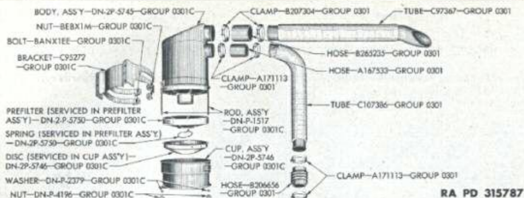
FIGURE 03-5—AIR CLEANER—ROUND TYPE—WITH TUBE AND HOSE CONNECTIONS
