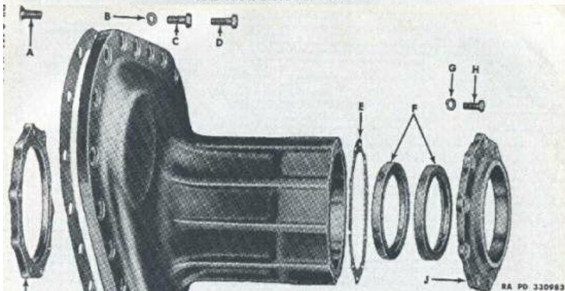
FIGURE 10-4—FINAL DRIVE COVER, CAPS AND OIL SEALS
