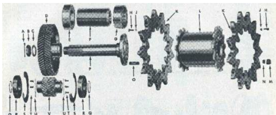
FIGURE 10-5—FINAL DRIVE GEARS, HUB AND SPROCKETS
