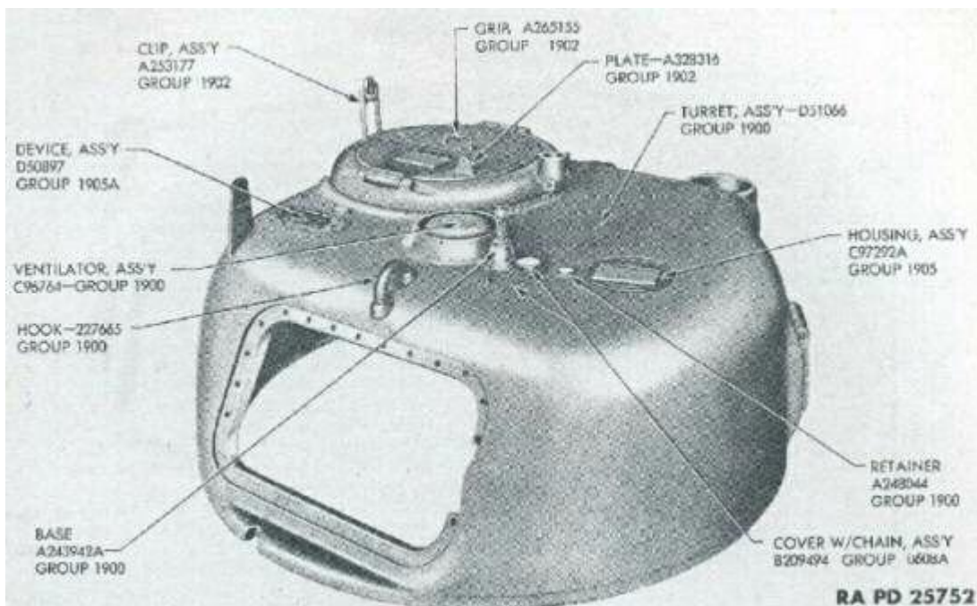
FIGURE 19-2 - TURRET ASSEMBLY - UPPER FRONT VIEW
