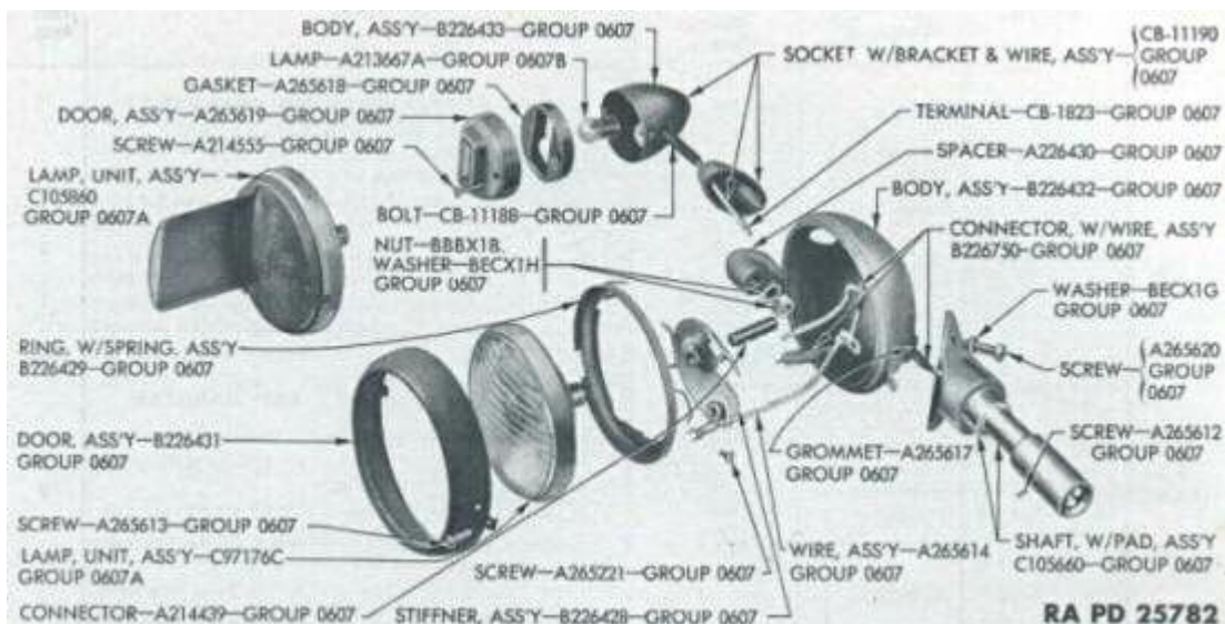
FIGURE 06-6 - HEADLIGHT AND BLACKOUT LIGHT ASSEMBLY - EXPLODED VIEW
