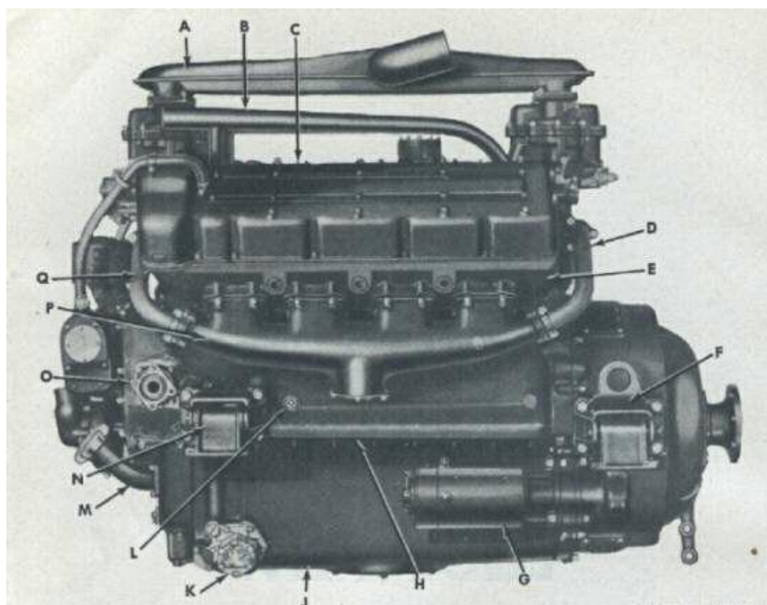
FIGURE 01-1—GASOLINE ENGINE—RIGHT SIDE VIEW
