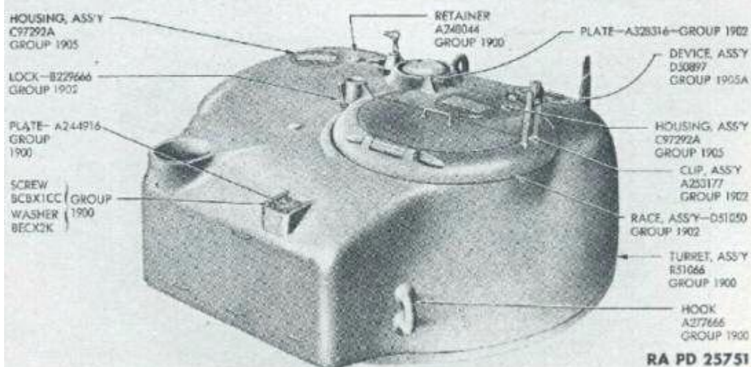
FIGURE 19-3 - TURRET ASSEMBLY - UPPER REAR VIEW
