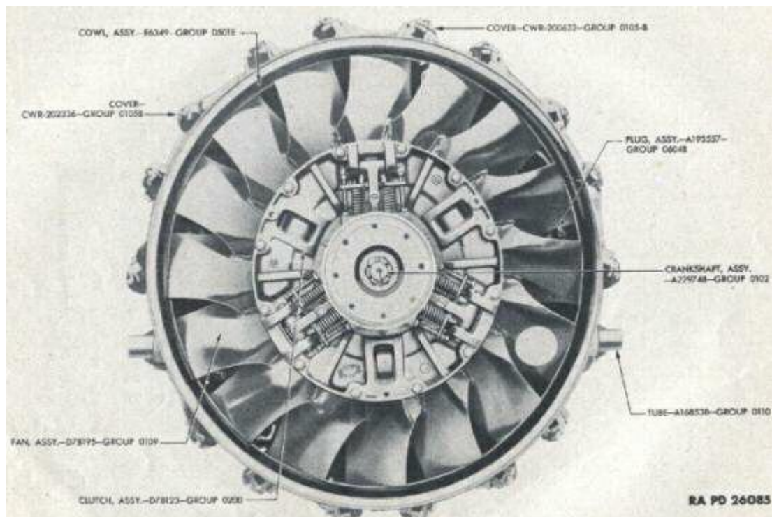
FIGURE 01-4—ENGINE ASSEMBLY—FRONT VIEW (USED ON LATE MODEL TANK, MEDIUM, M4, M4A1 AND ALL M4 105-MM HOWITZER)
