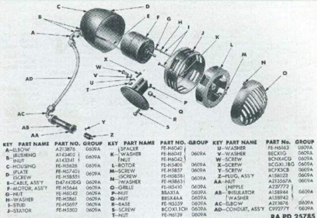
FIGURE 06-9 - SIREN ASSEMBLY - EXPLODED VIEW
