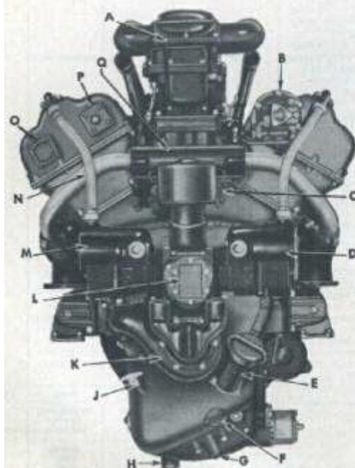
FIGURE 06-56—AUXILIARY GENERATOR INSTALLATION (EARLY TYPE)
