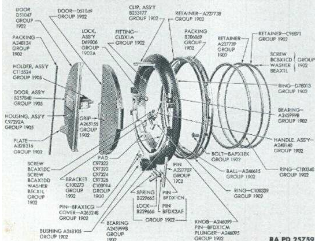
FIGURE 19-7 - TURRET HATCH RACE ASSEMBLY - EXPLODED VIEW
