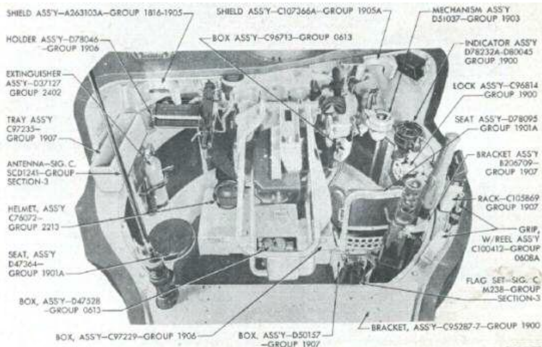
FIGURE 19-3 - TURRET AND PLATFORM - CUT-AWAY VIEW
