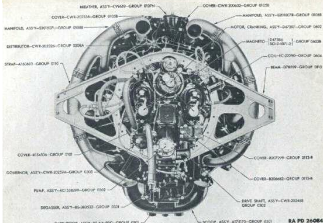
FIGURE 01-3—ENGINE ASSEMBLY—REAR VIEW—USED ON LATER MODEL TANK, MEDIUM, M4, M4A1 AND ALL M4 (105 MM HOWITZER)
