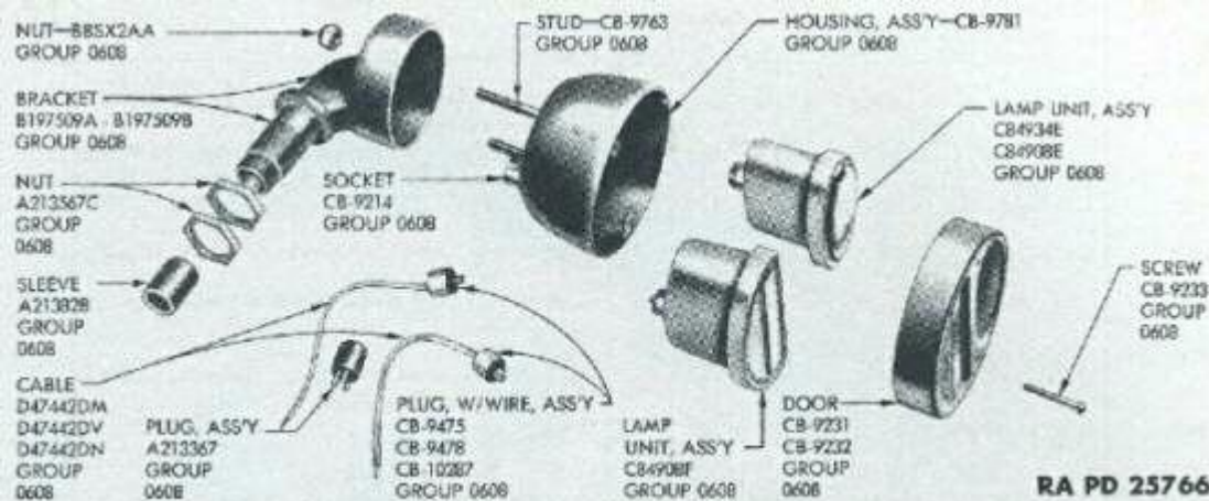
FIGURE 06-7 - TAIL LIGHT ASSEMBLY, LEFT AND RIGHT - EXPLODED VIEW
