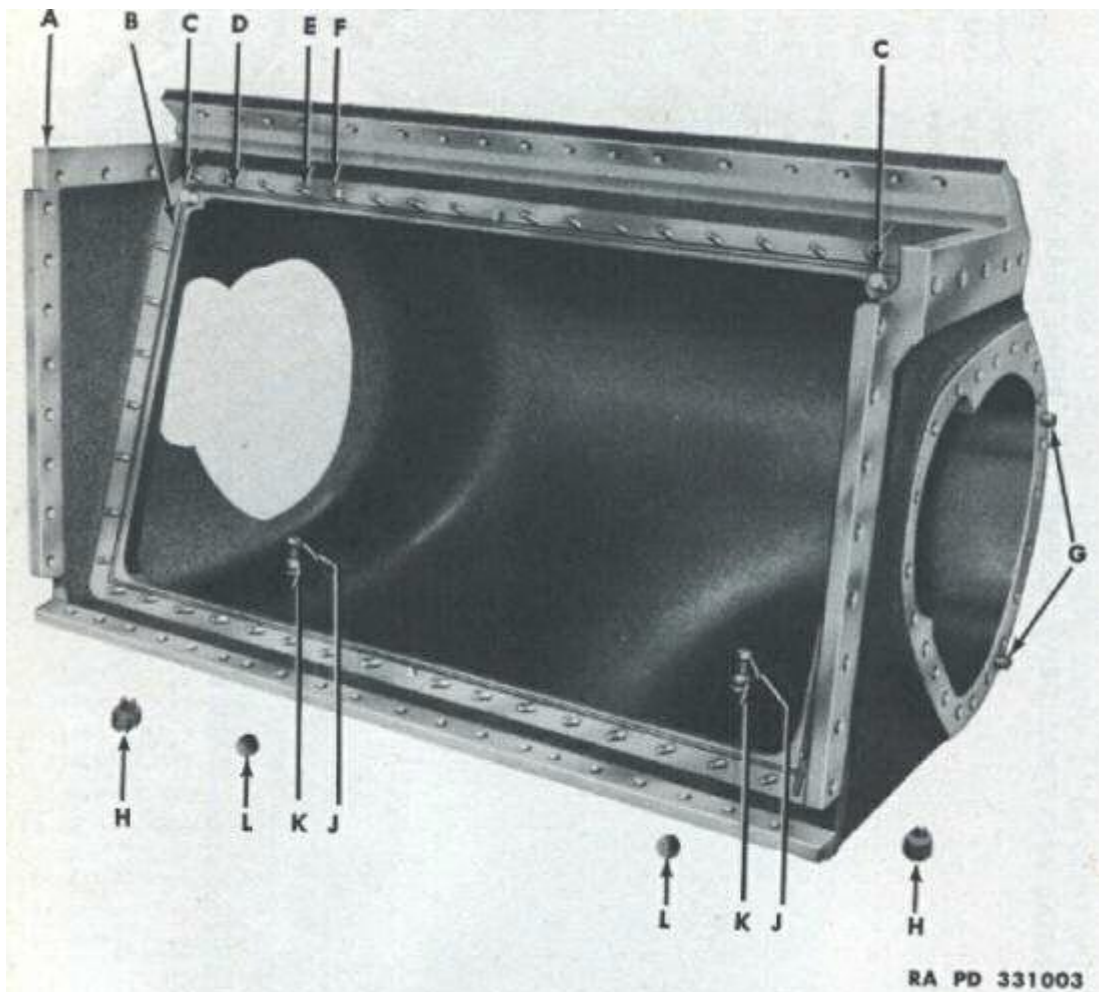
FIGURE 10-2—DIFFERENTIAL HOUSING
