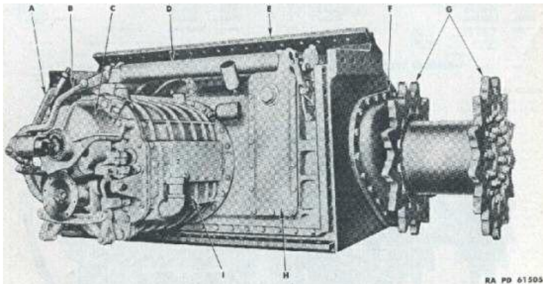
FIGURE 10-12—TRANSMISSION W/PARKING BRAKE, DIFFERENTIAL (SINGLE ANCHOR BRAKE) AND FINAL DRIVE ASSEMBLIES
