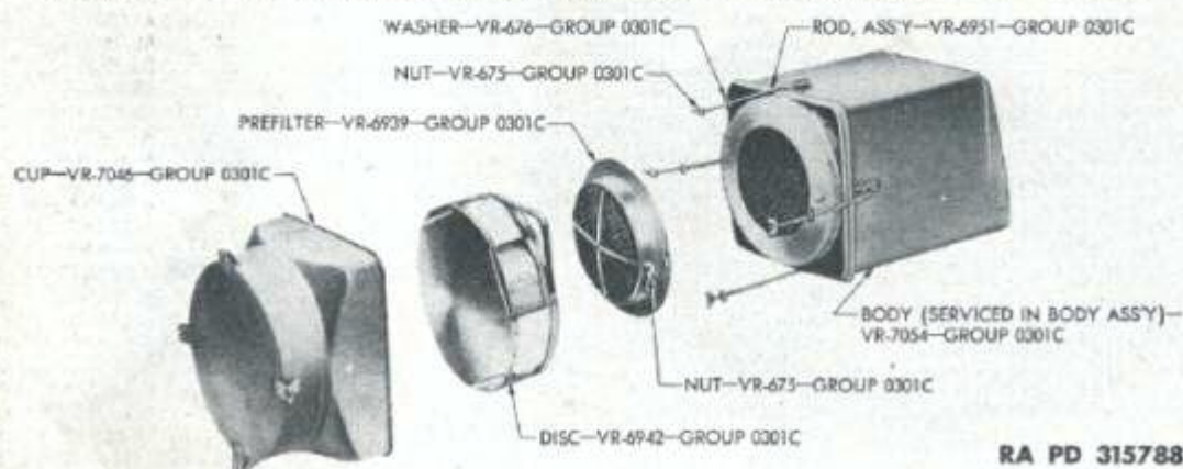
FIGURE 03-6—AIR CLEANER—SQUARE TYPE
